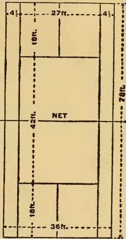
Fig. 25.—Tennis court
